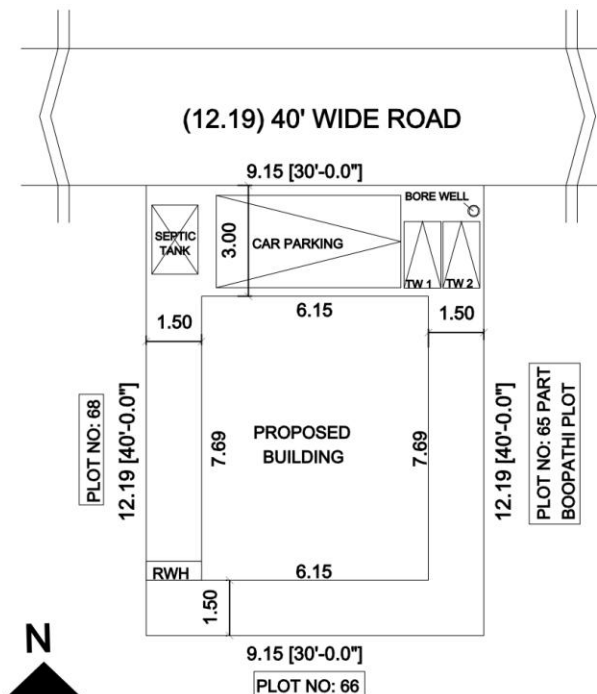
SITE PLAN
