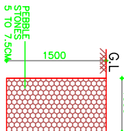
SECTION OF PEBBLE TRENCH SCALE : 1" = 100
