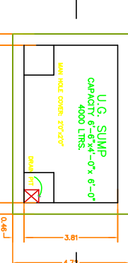
SECTION ON D-D
