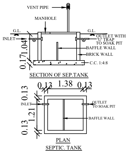
PLAN SEPTIC TANK
