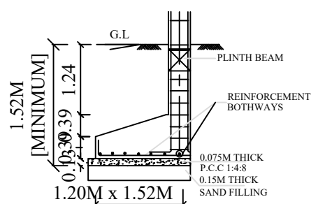
TYP. DET. ECCENTRIC COLUMN FOOTING
