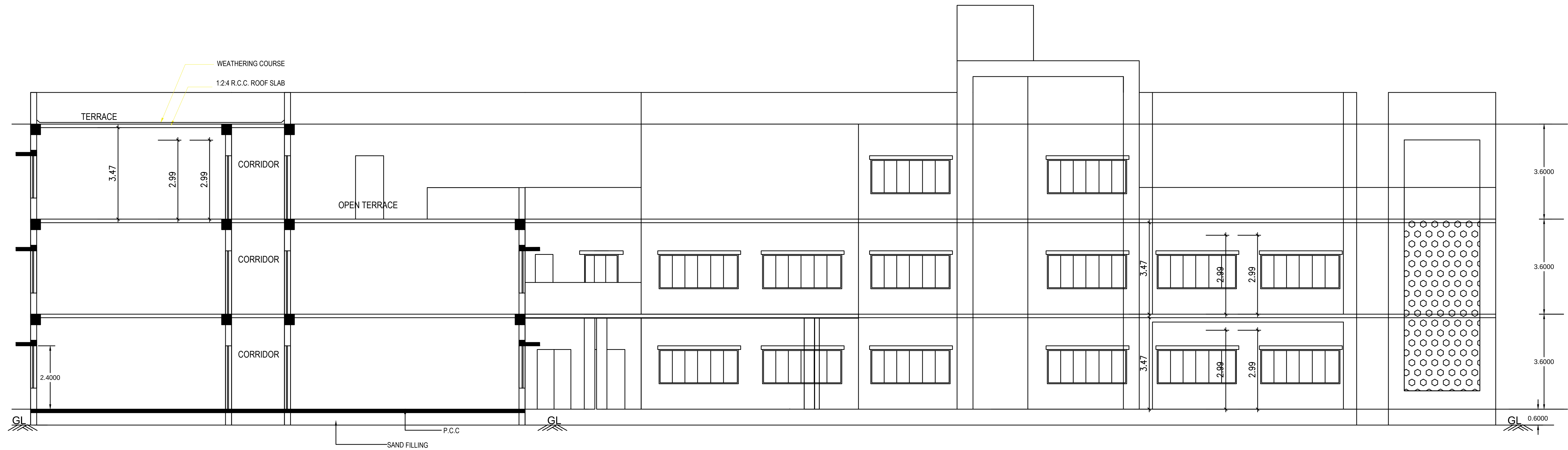
SECTION ON AA
