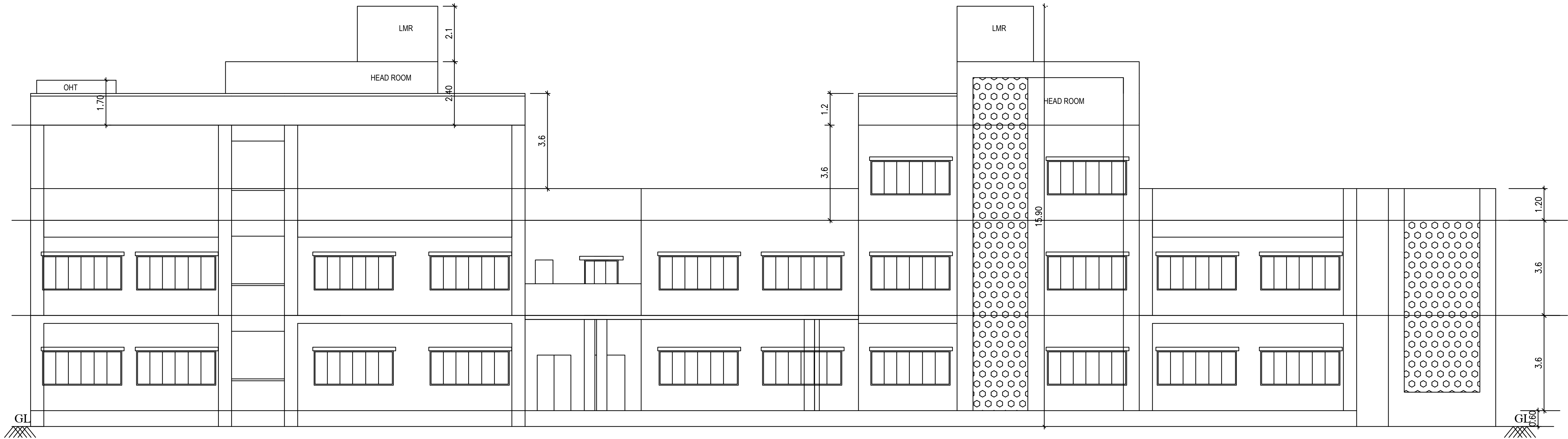
FRONT ELEVATION (EAST FACING)
