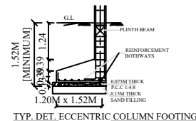
TYP. DET. ECCENTRIC COLUMN FOOTING
