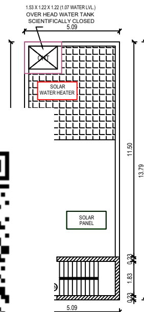
THE FLOOR PLAN
