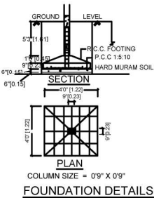
FOUNDATION DETAILS
