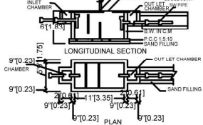
SEPTIC TANK:
