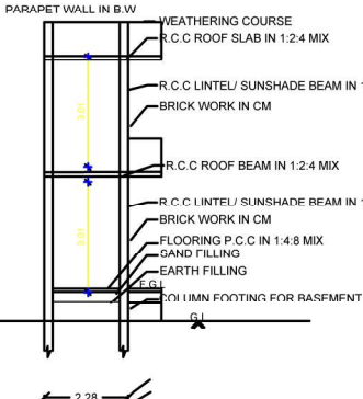
SECTION ON X-X
