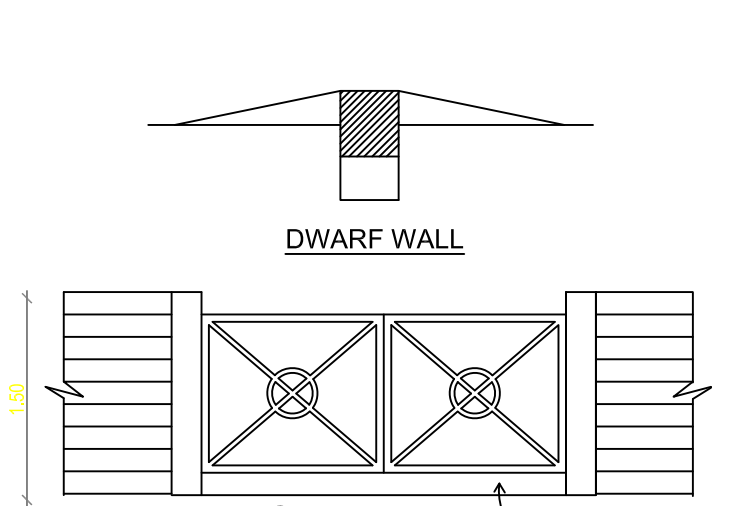
Gate Detail
