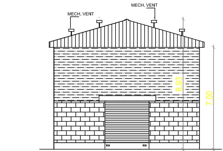
FRONT ELEVATION 16.0 M ( 52'-6" )
