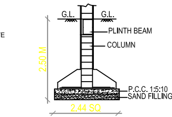
FOUNDATION DETAIL
