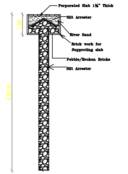
PERCOLATION PIT
