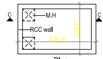
Plan Typical U.G Sump
