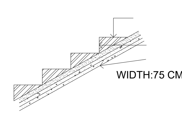
CROSS SECTION OF STAIRCASE
