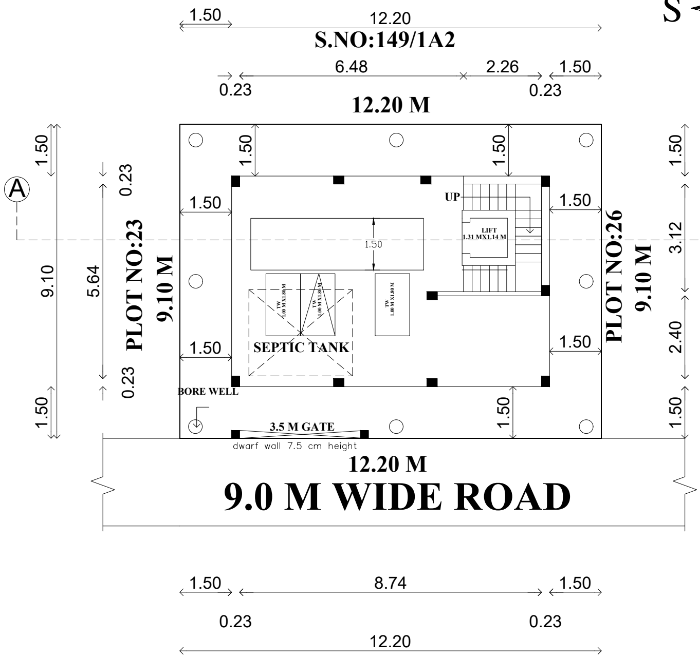
SITE PLAN CUM STILT FLOOR PLAN
