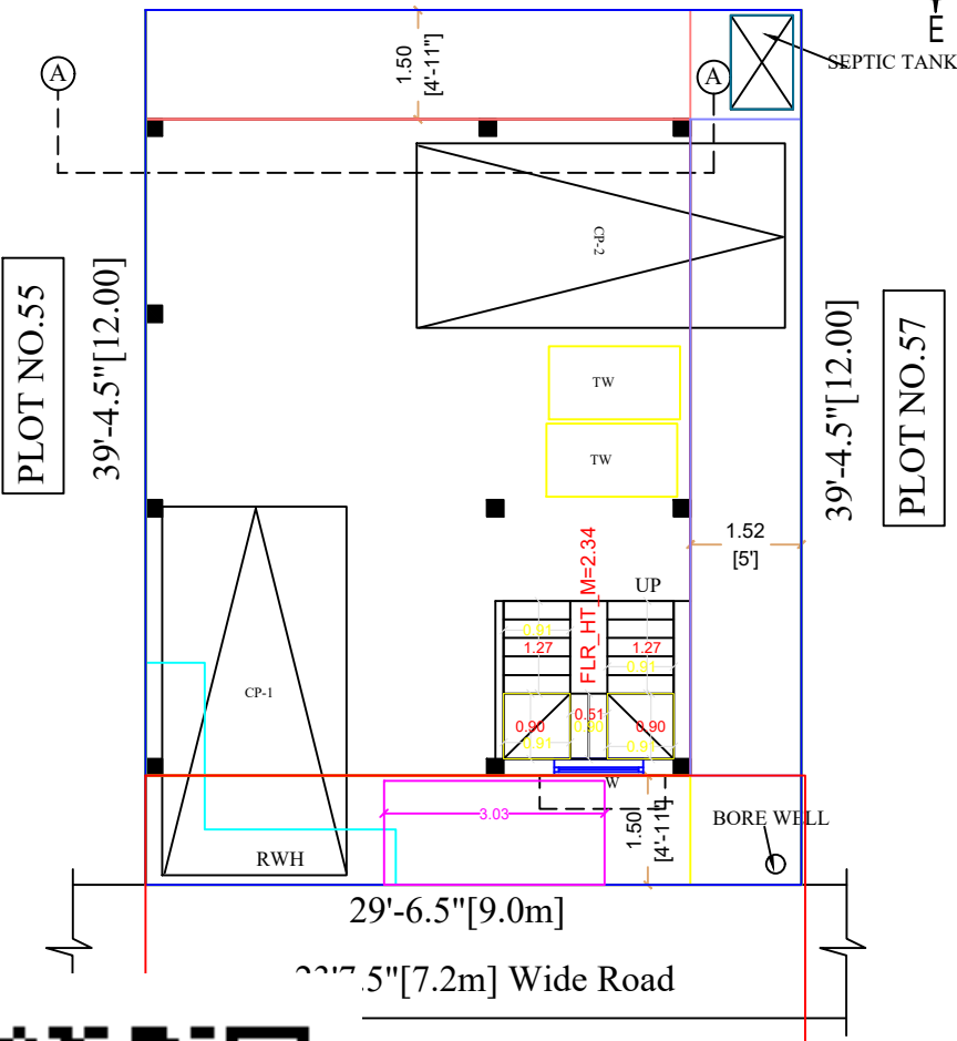
RO. STILT FLOOR PLAN
