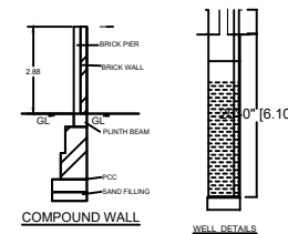
COMPOUND WALL
