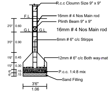
COLUMN DETAIL
