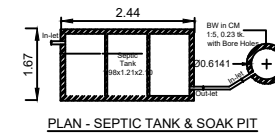
PLAN - SEPTIC TANK & SOAK PIT
