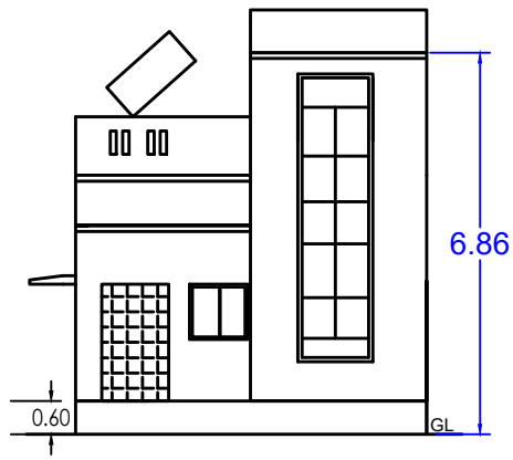
FRONT ELEVATION
