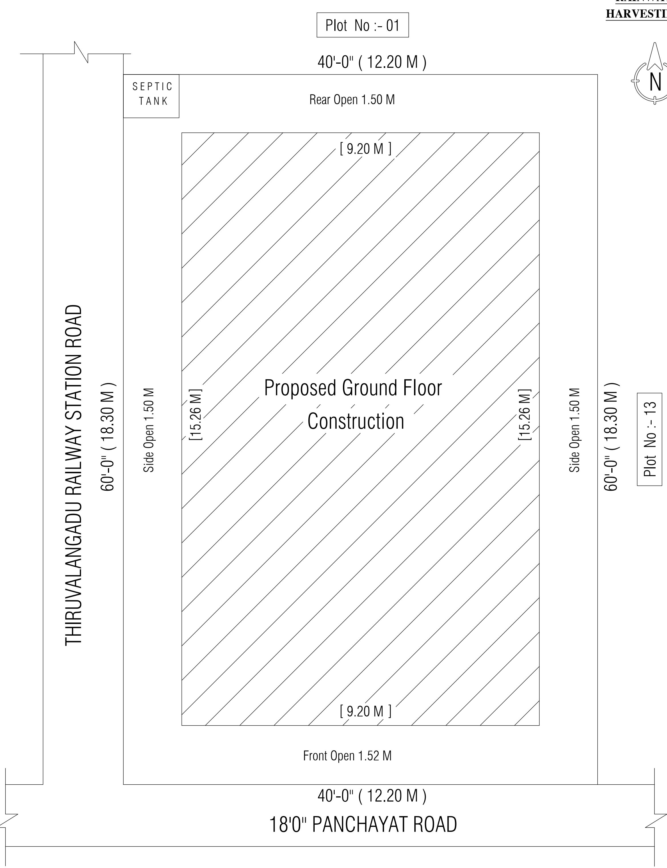
SITE PLAN
