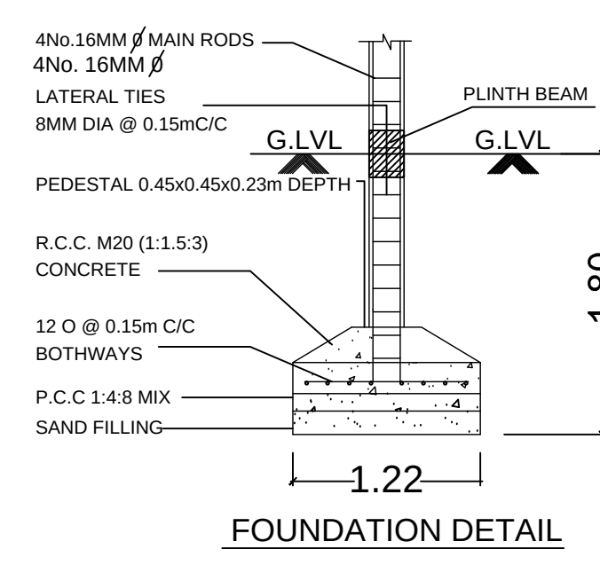
FOUNDATION DETAIL
