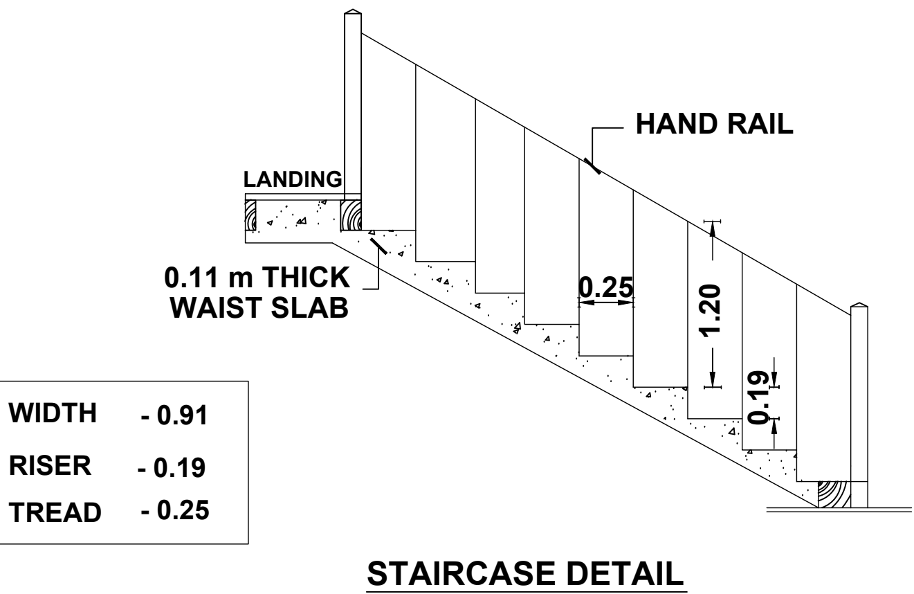
STAIRCASE DETAIL
