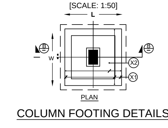
FOUNDATION DETAIL
