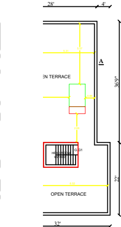
TERRACE FLOOR PLAN
