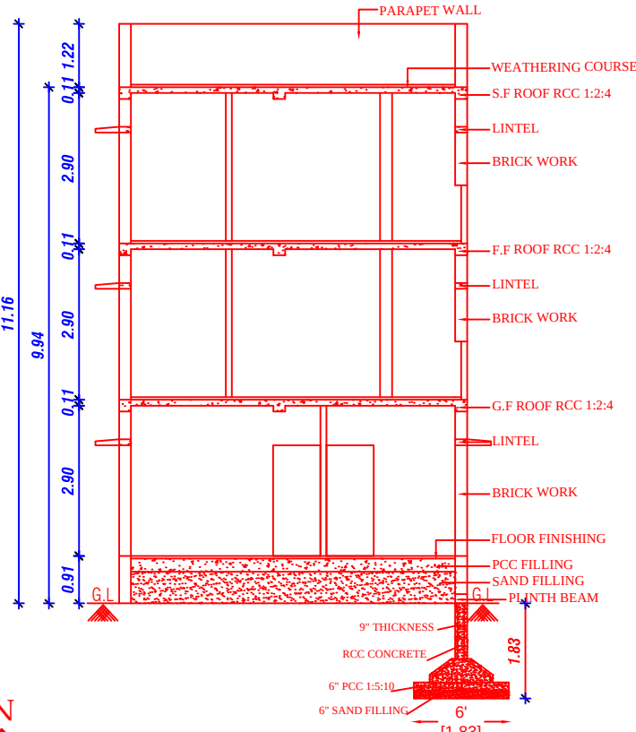
CROSS SECTION ON [A-A]
