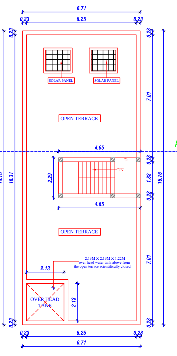
OPEN TERRACE FLOOR PLAN
