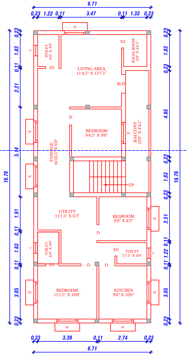
PRO.SECOND FLOOR PLAN
