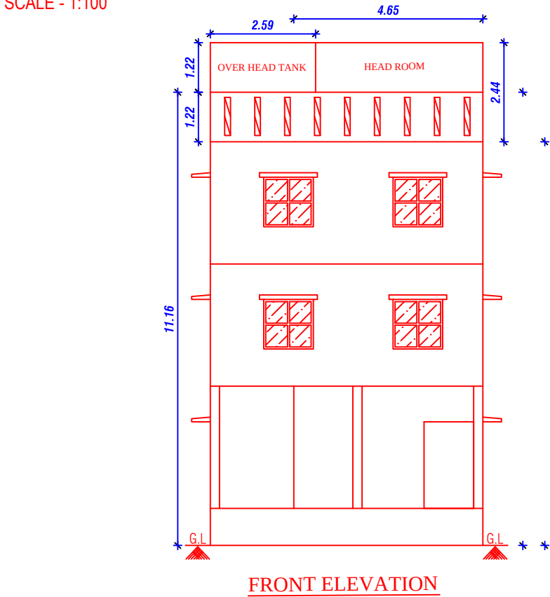
FRONT ELEVATION
