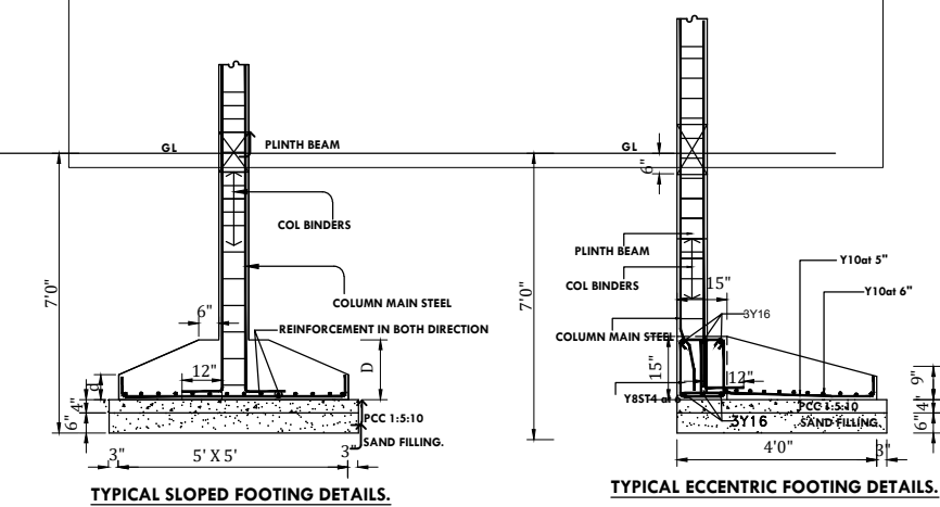
TYPICAL SLOPED FOOTING DETAILS.
