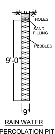
WELL DETAILS
