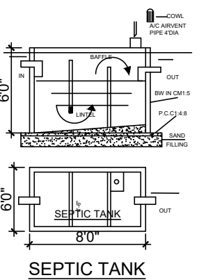
SEPTIC TANK
