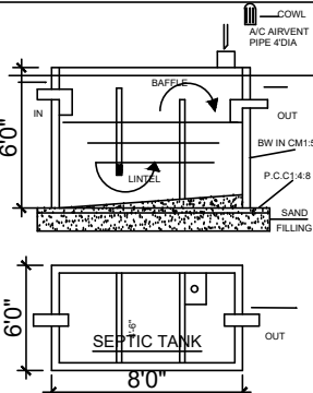
SEPTIC TANK
