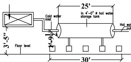
SOLAR HOT WATER SYSTEM(SWHS) DETAIL
