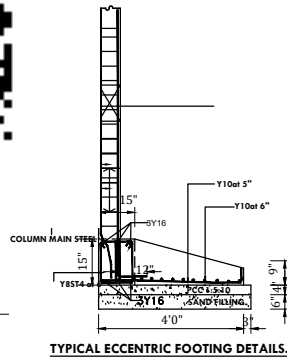
TYPICAL ECCENTRIC FOOTING DETAILS.
