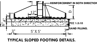
TYPICAL SLOPED FOOTING DETAILS.
