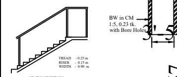
STAIRCASE DETAILS
