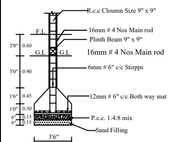
COLUMN DETIAL
