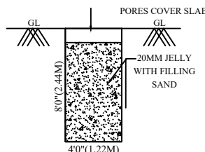
RAINWATER HARVESTING UNIT
