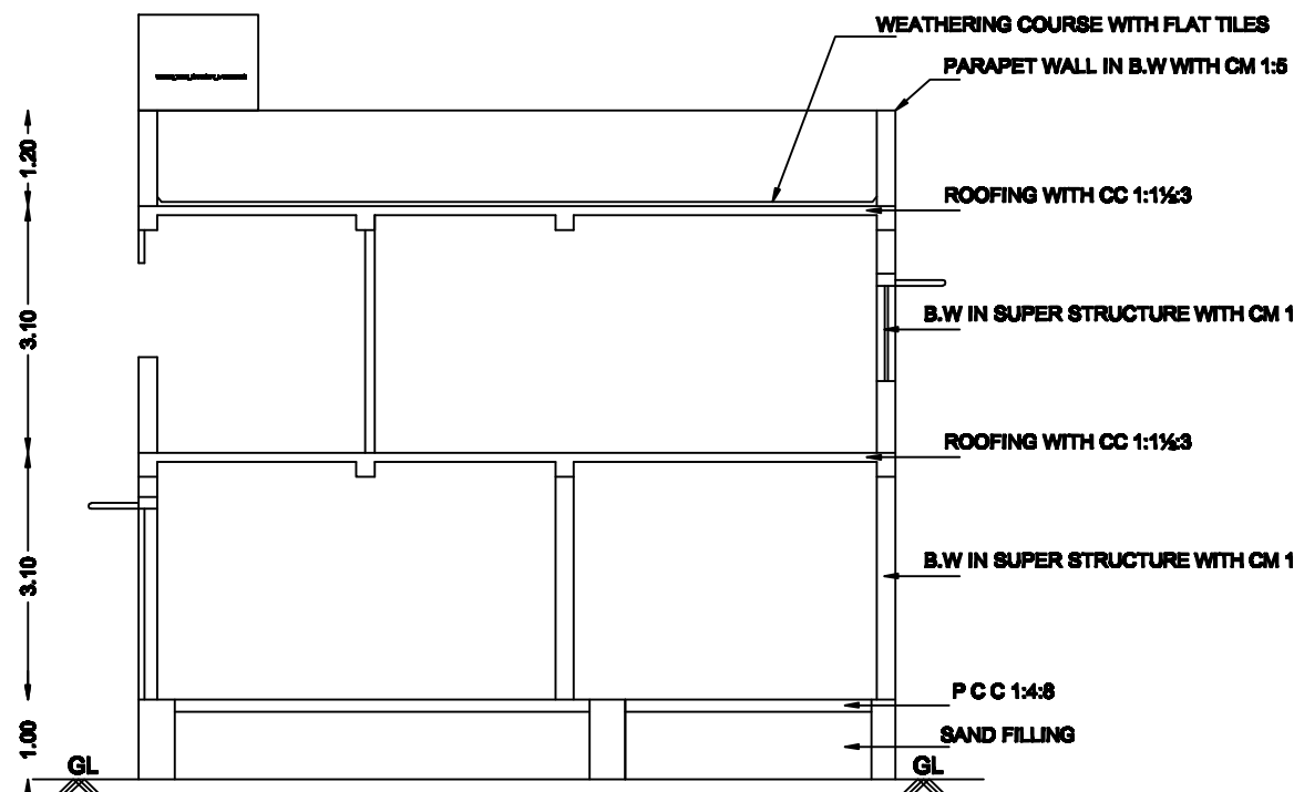
SECTION ON R-J
