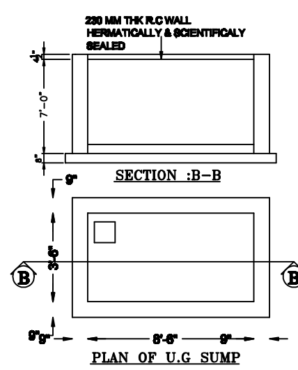
PLAN OF U.G SUMP
