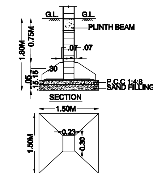
COLUMN PLAN SIZE: 0.23X0.30 TYPICAL FOUNDATION DETAIL
