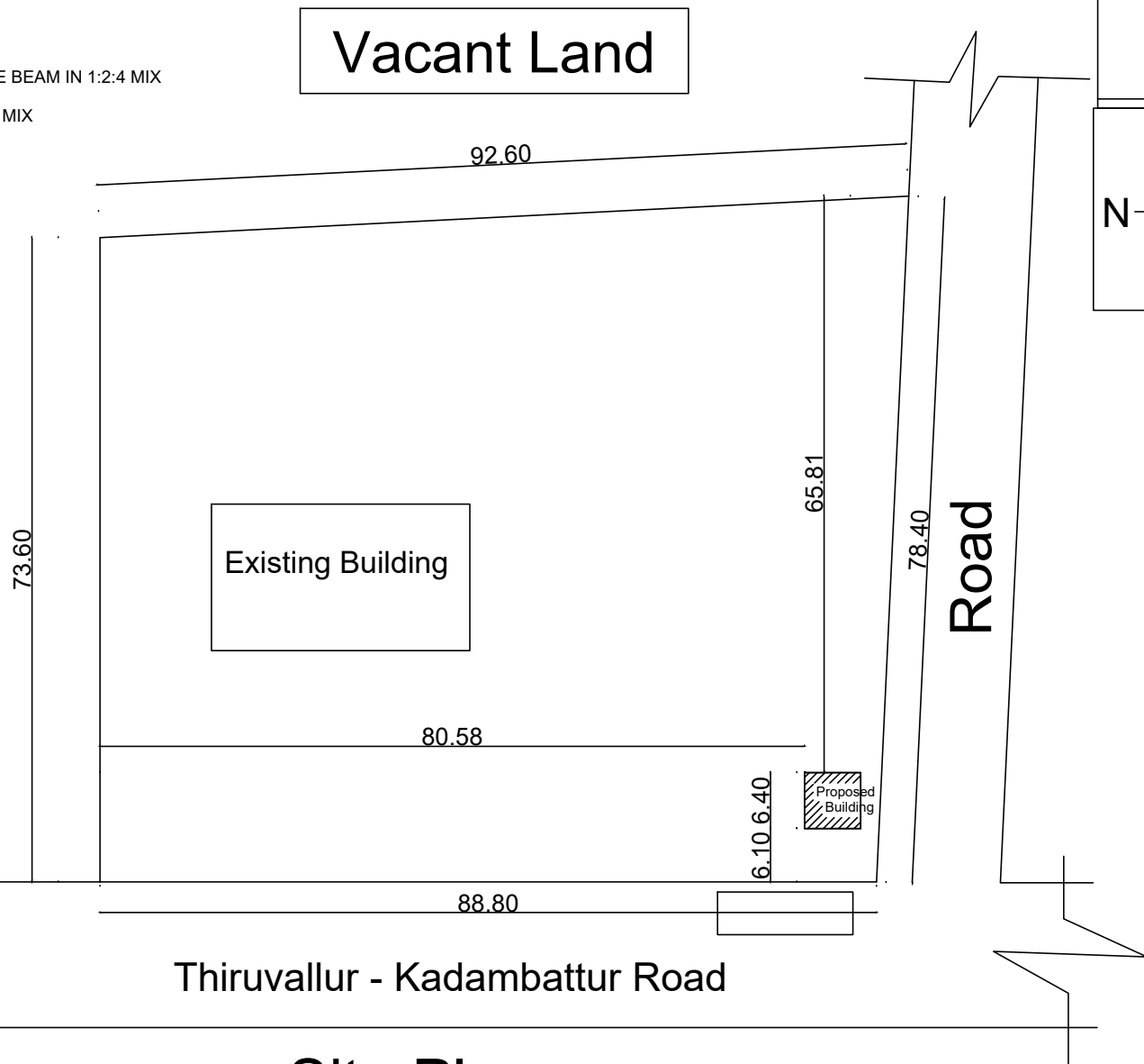
Site Plan
