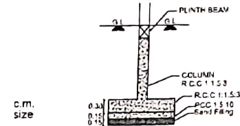
Foundation Details
