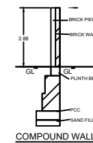
COMPOUND WALL
