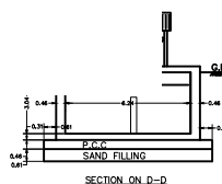
SECTION ON D-D
