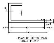
PLAN OF SEPTIC TANK SCALE 1"=2'0"
