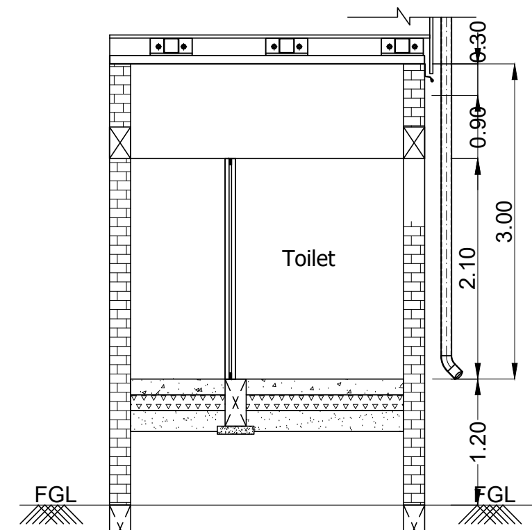
SECTION B-B
