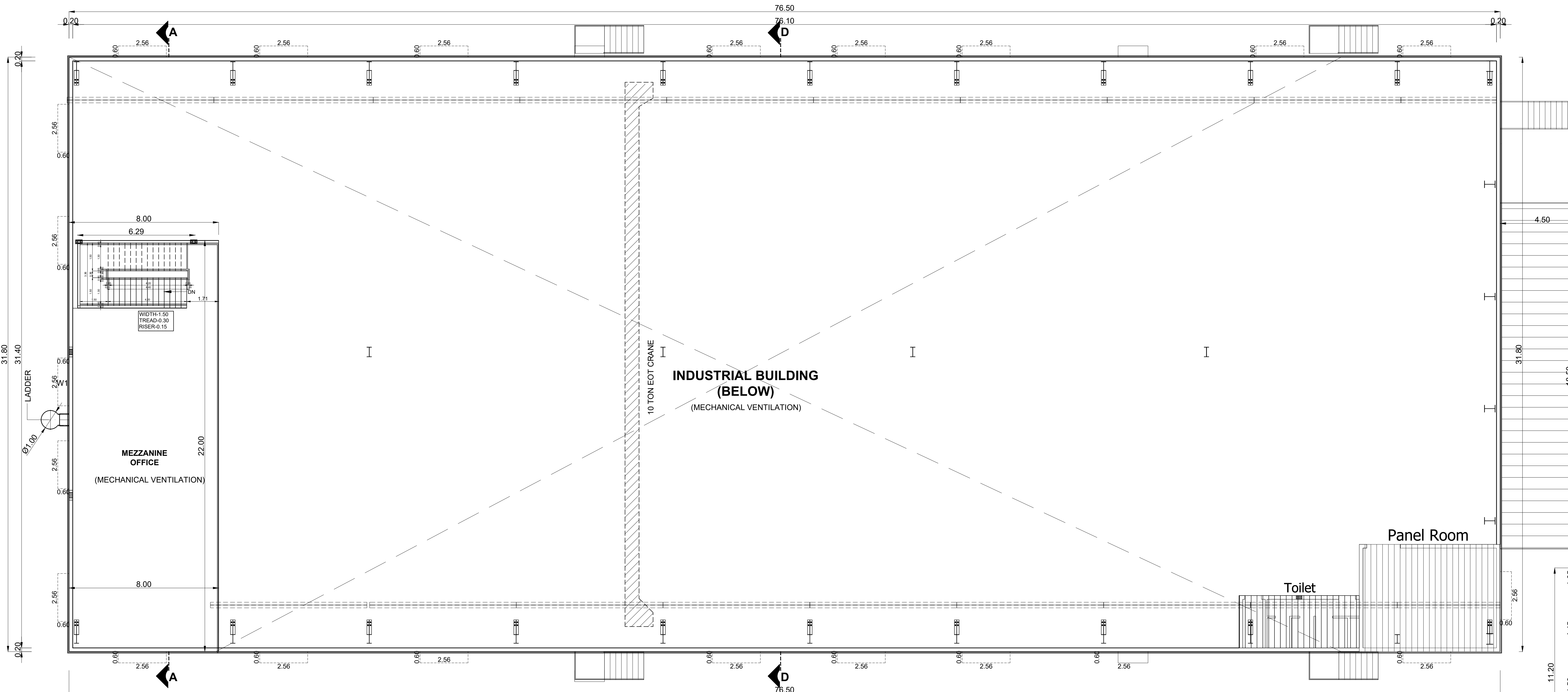
MEZZANINE FLOOR PLAN
