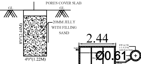
RAINWATER HARVESTING UNIT
