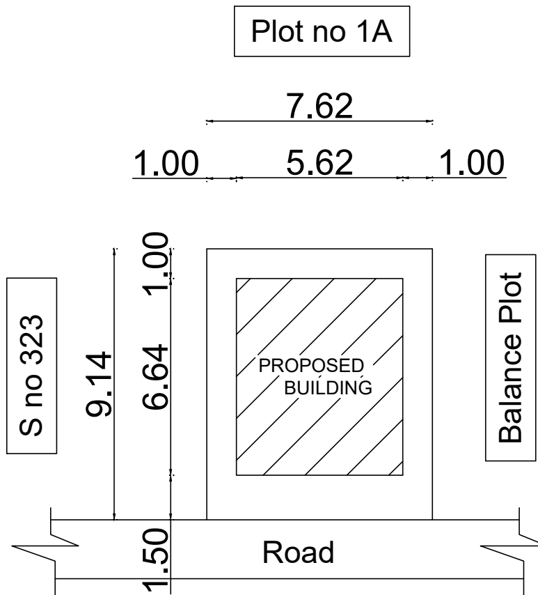
Site Plan
