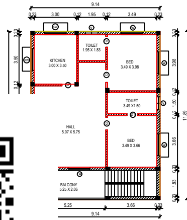
IRST FLOOR PLAN
