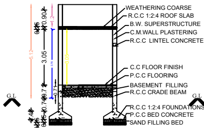
BLOCK-3 SECTION ON AA
