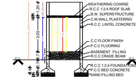
BLOCK-2 SECTION ON AA
