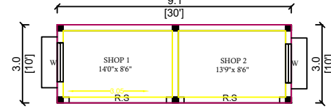
BLOCK-1 GROUND FLOOR PLAN
