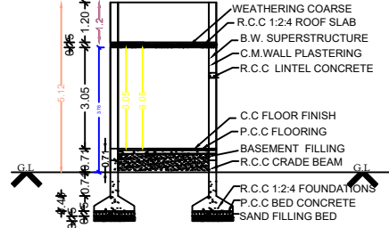
BLOCK-1 SECTION ON AA
