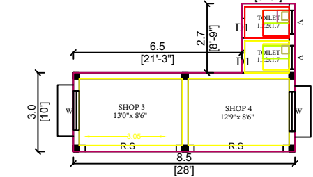
BLOCK-2 GROUND FLOOR PLAN
