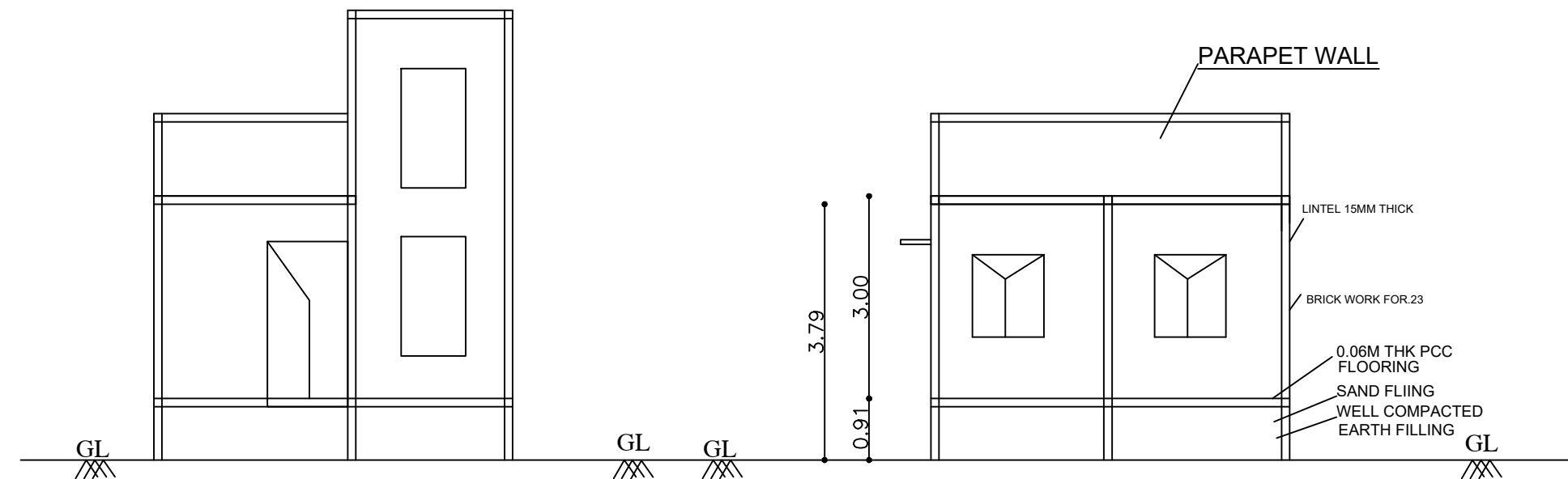
SECTION-AA
