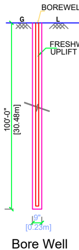
Bore Well
