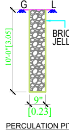
PERCOLATION PIT
