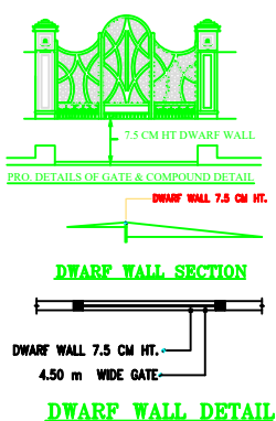
DWARP WALL DETAIL
