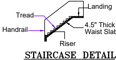
STAIRCASE DETAIL
