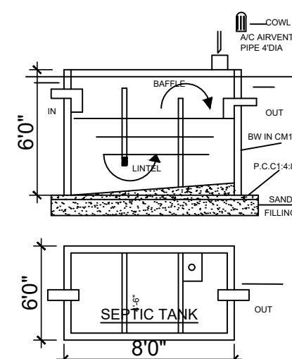
SEPTIC TANK
