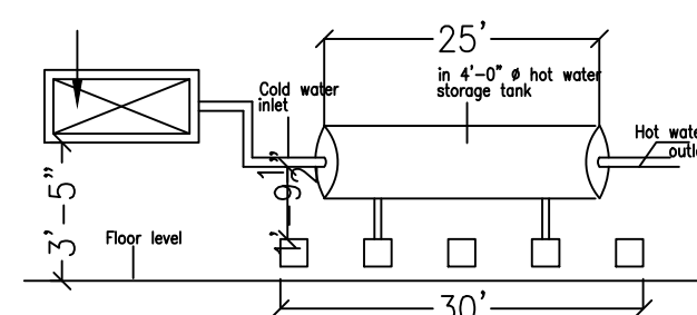
SOLAR HOT WATER SYSTEM(SWHS) DETAIL
