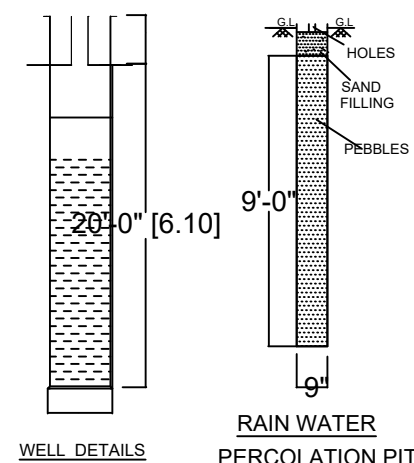
WELL DETAILS
