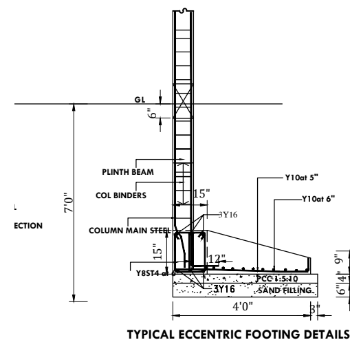
TYPICAL ECCENTRIC FOOTING DETAILS
