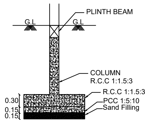
Foundation Details
