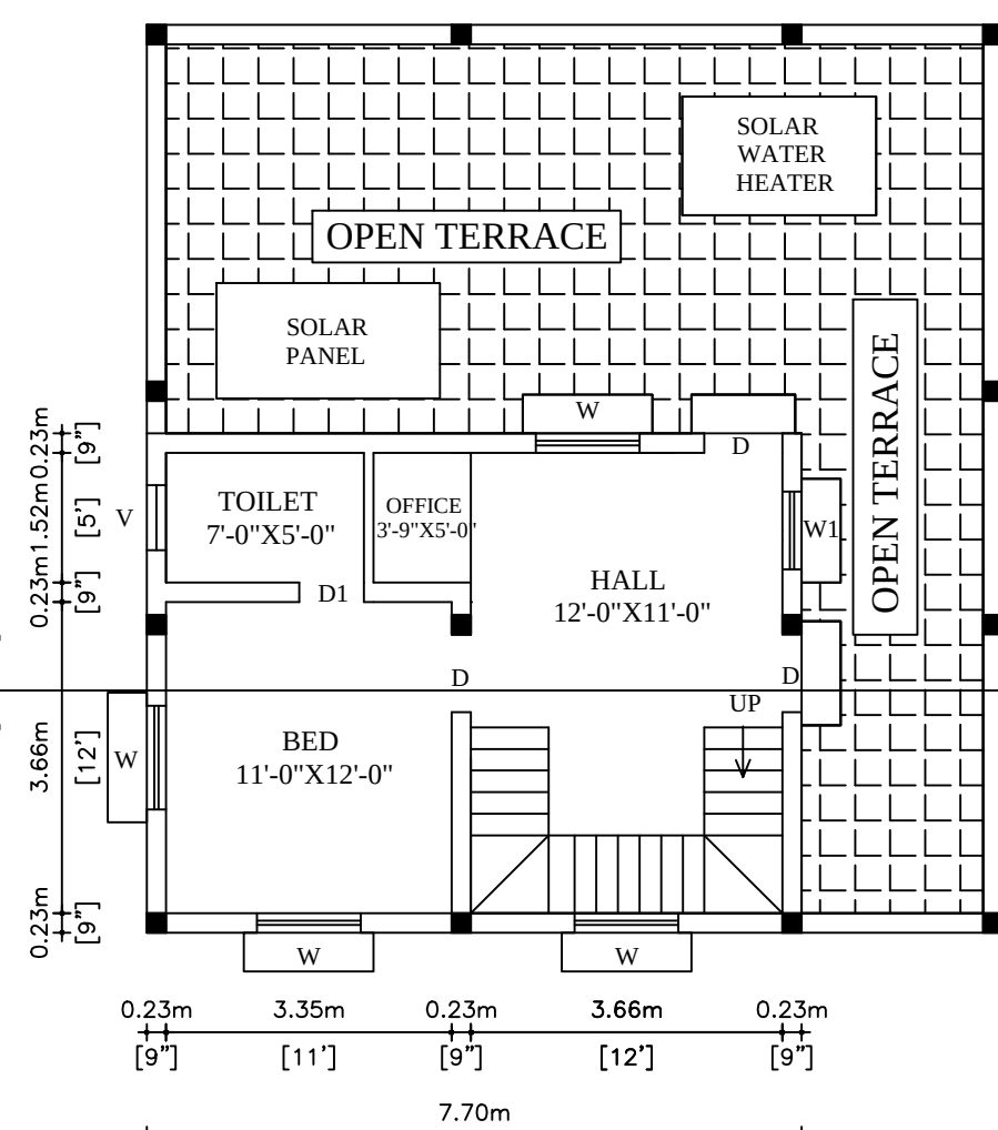
FIRST FLOOR (PART) PLAN
