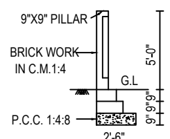
SECTION 2-0
