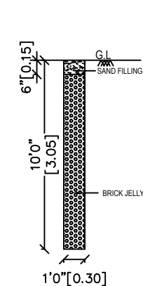
RAIN WATER PERCOLATION PIT
