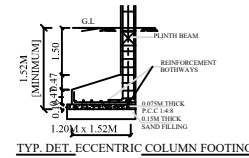
TYP. DET. ECCENTRIC COLUMN FOOTING
