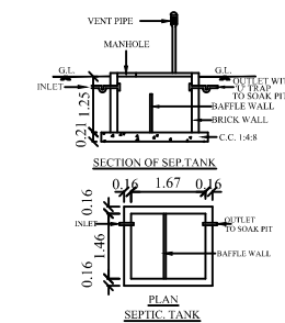
PLAN SEPTIC TANK
