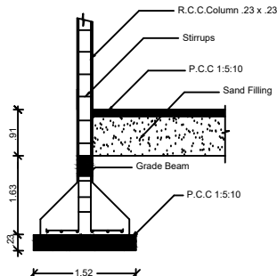
COLUMN DETAIL
