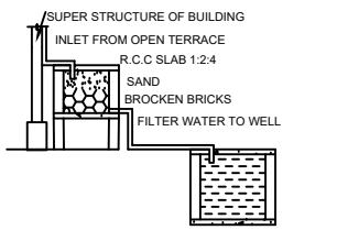
RAINWATER HARVESTING
