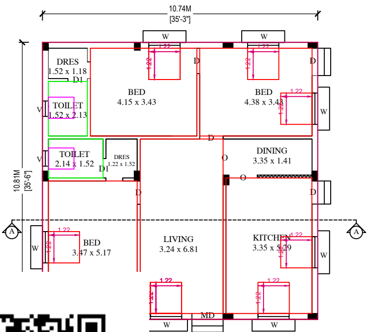
ND FLOOR PLAN
