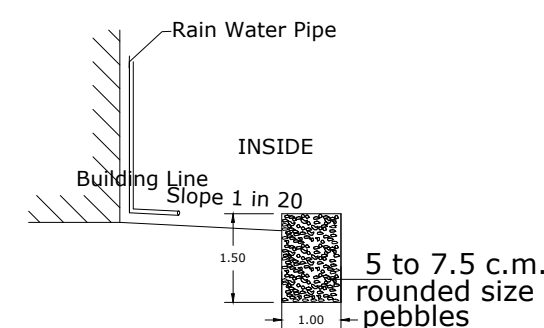
RAINWATER HARVESTING
