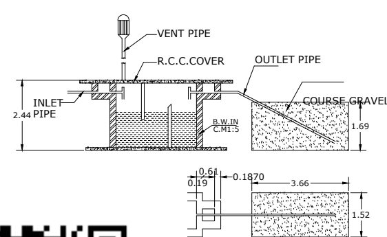
3 DISPERSION DETAILS
