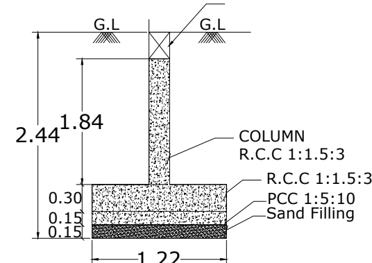
FOUNDATION DETAILS
