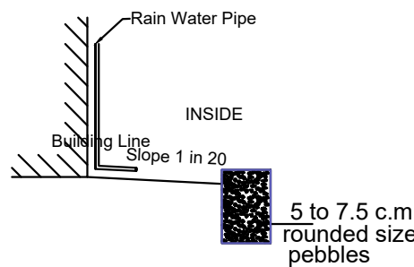
RAINWATER HARVESTING
