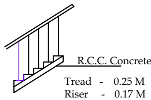
Staircase details
