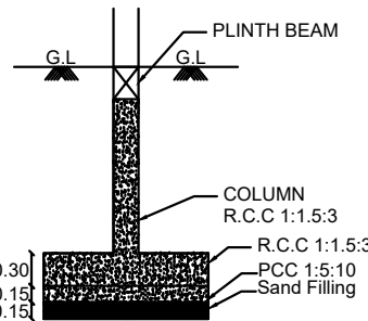
Foundation Details
