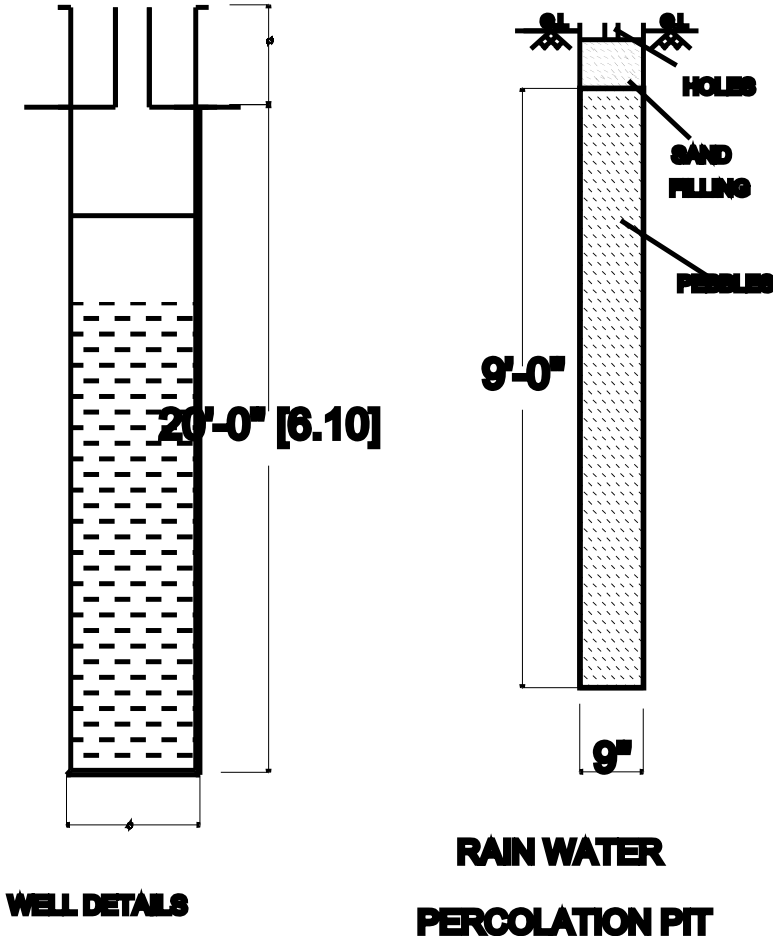
WELL DETAILS RAIN WATER PERCOLATION PIT
