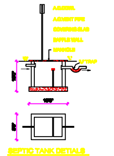
SEPTIC TANK DETAILS
