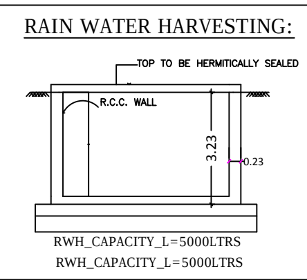
RAIN WATER HARVESTING: RWHL CAPACITY_L=5000LTRS RWHL CAPACITY_L=5000LTRS
