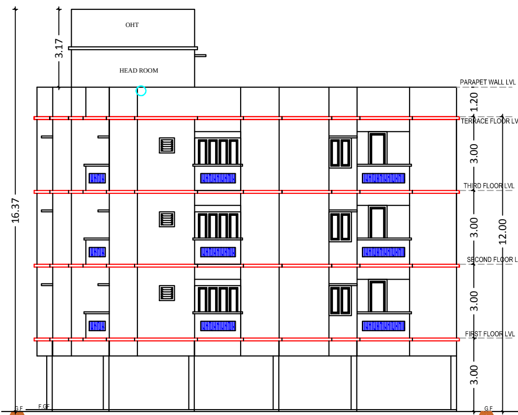
FRONT ELEVATION
