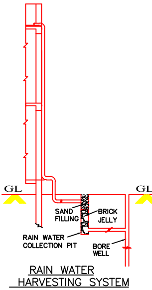
RAIN WATER HARVESTING SYSTEM
