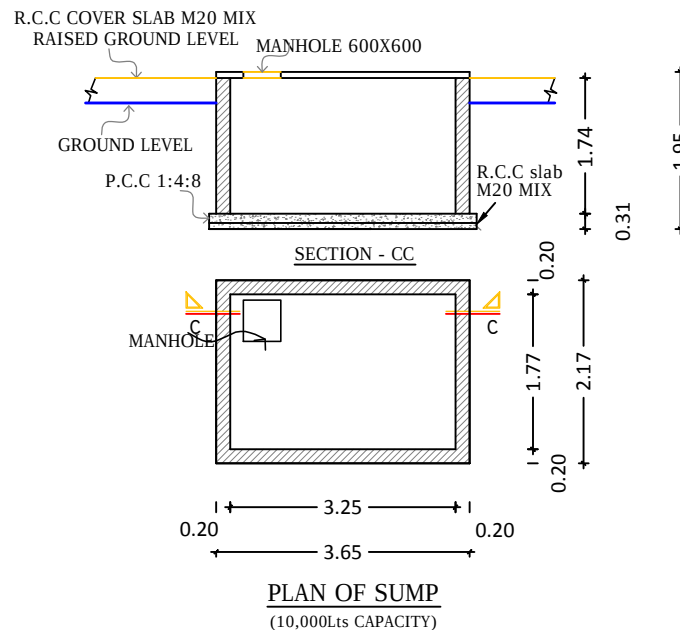
PLAN OF SUMP (10,000Ltr CAPACITY)
