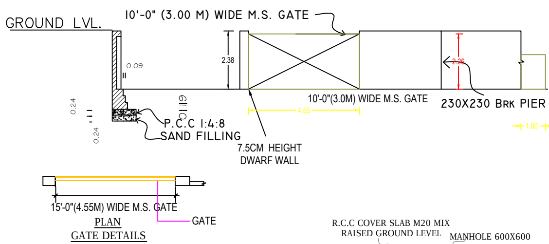
GATE DETAILS
