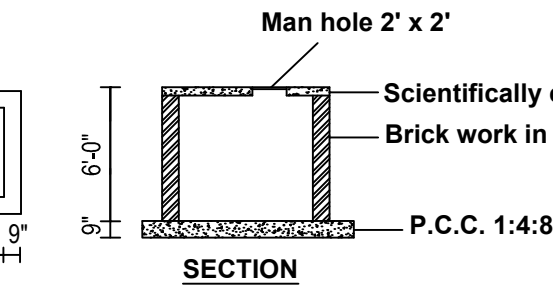
SUMP DETAIL
