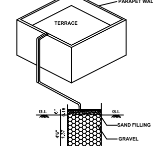
COLLECTION SUMP FOR RAIN WATER HARVESTING
