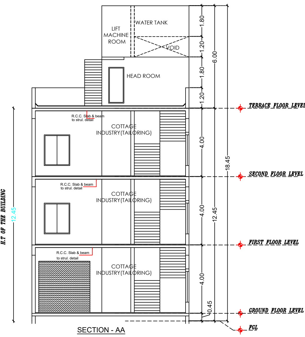
SECTION - AA
