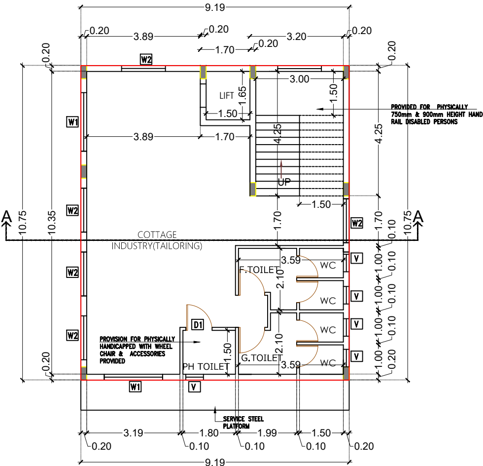
TYPICAL FLOOR PLAN (1ST & 2ND FLOORS)
