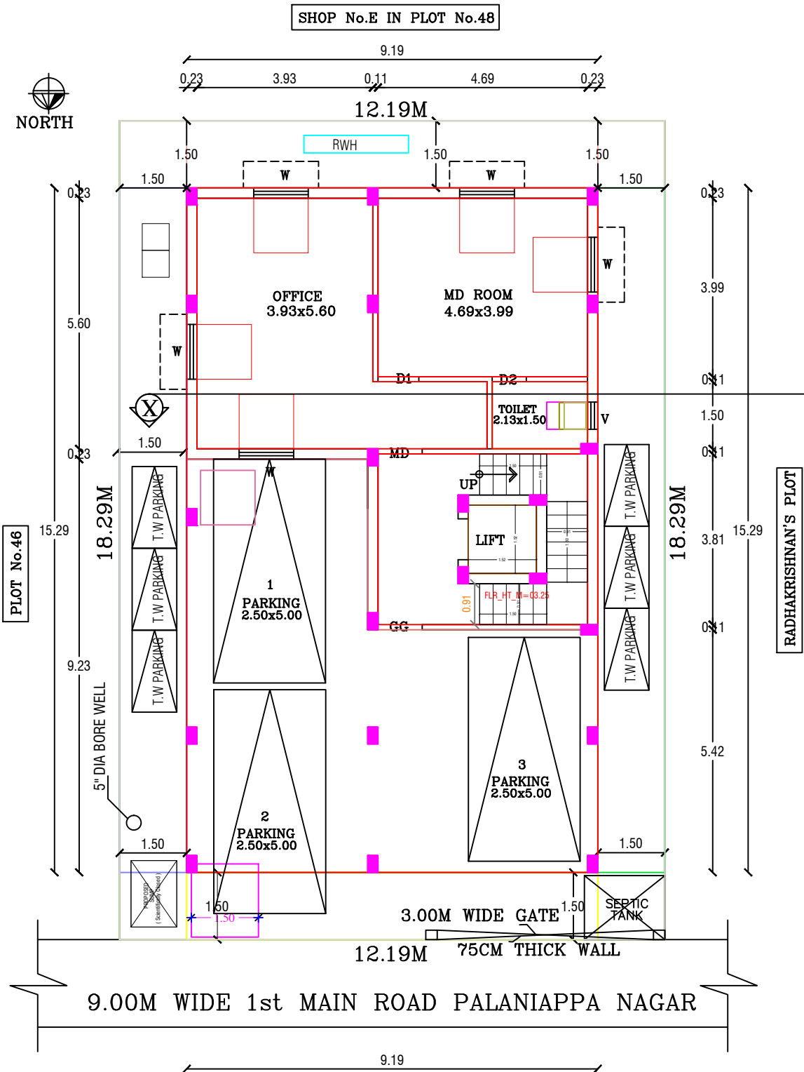
SITE CUM STILT & GROUND FLOOR PART PLAN (PROPOSED)
