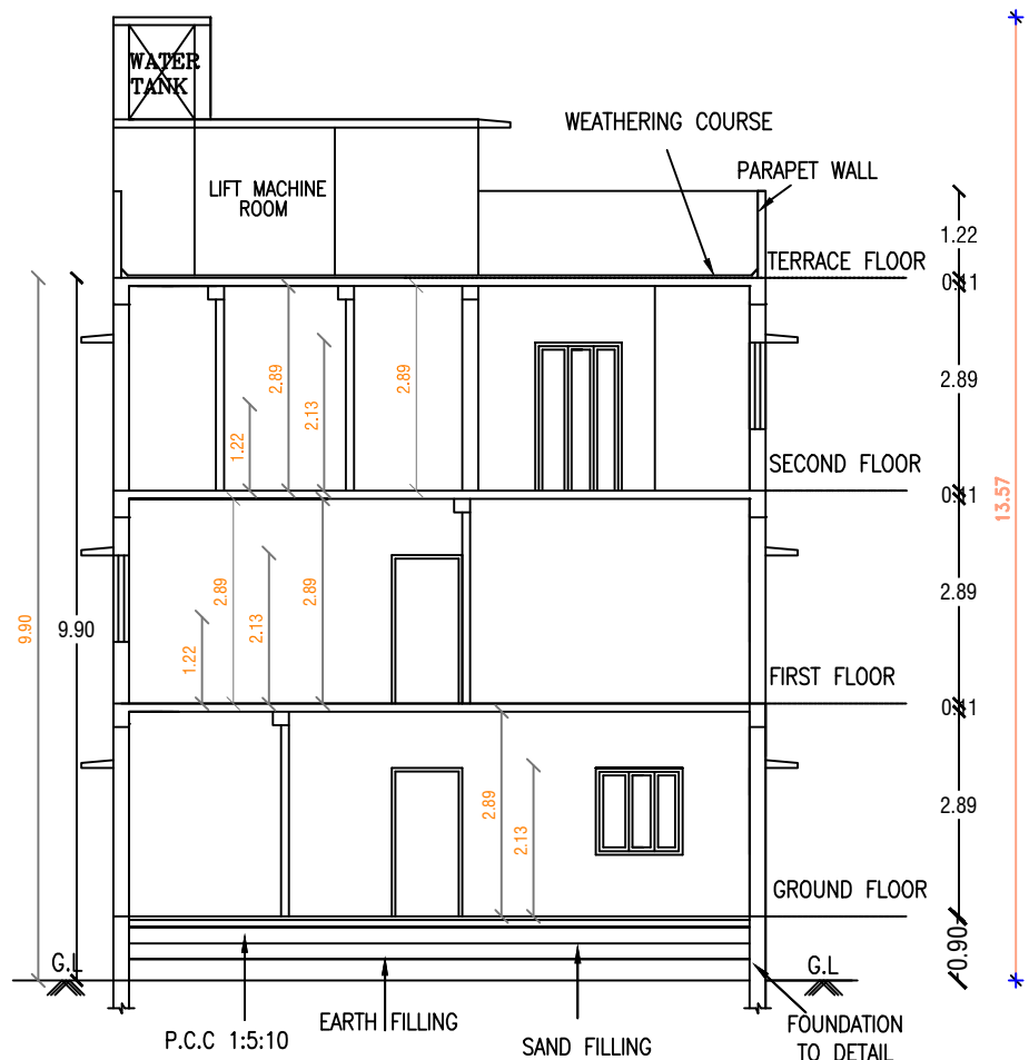
SECTION 'X-X'
