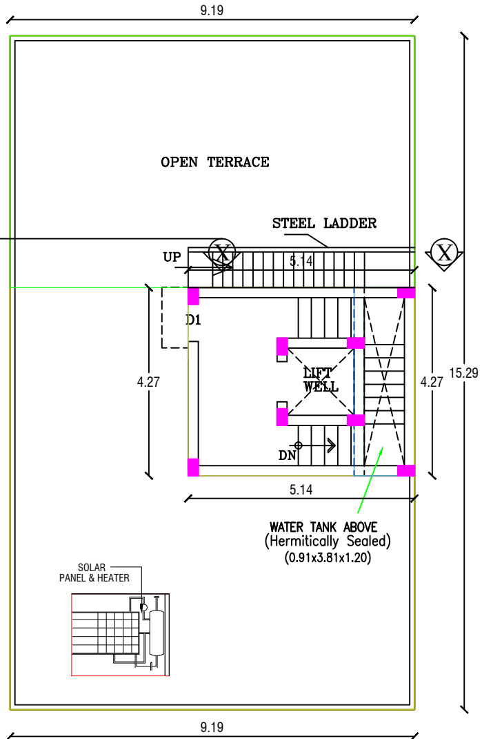
TERRACE FLOOR PLAN (PROPOSED)
