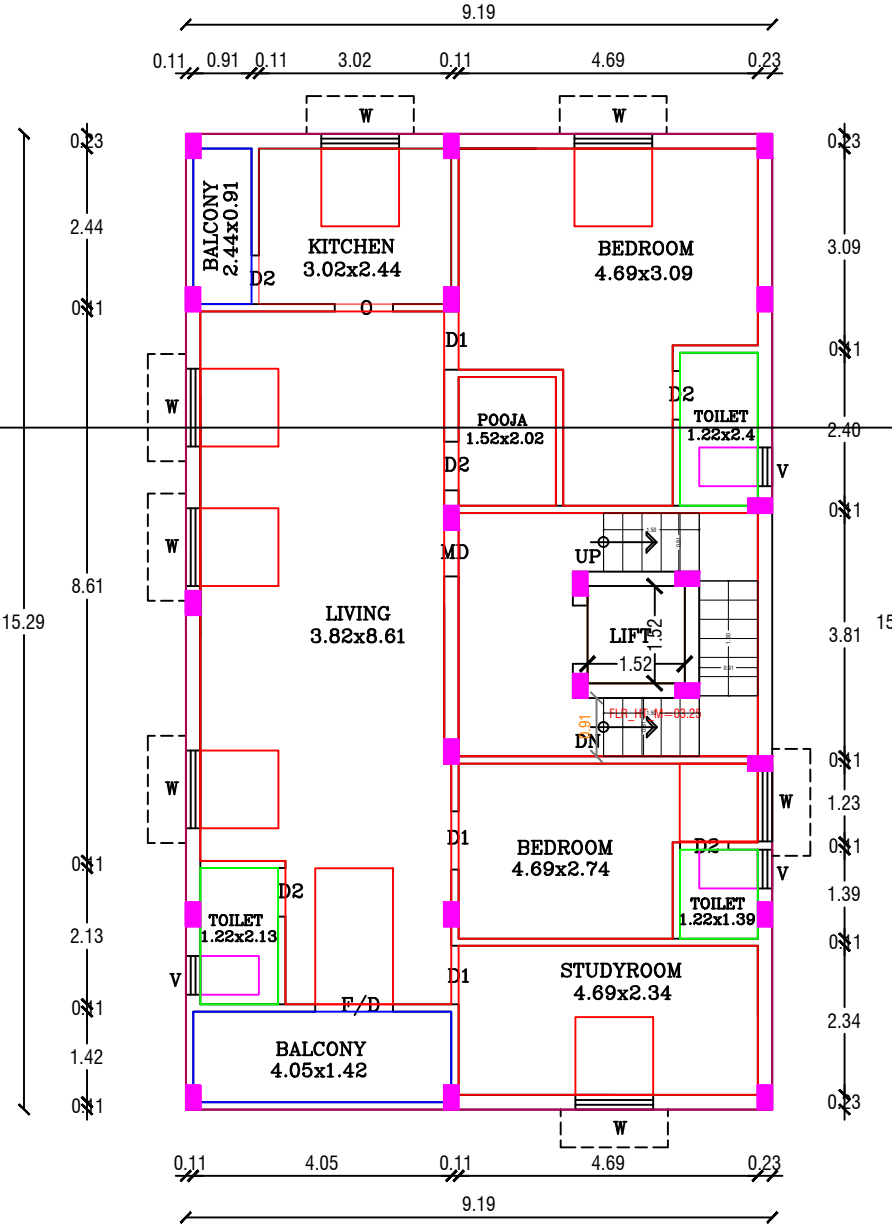
SECOND FLOOR PLAN (PROPOSED)
