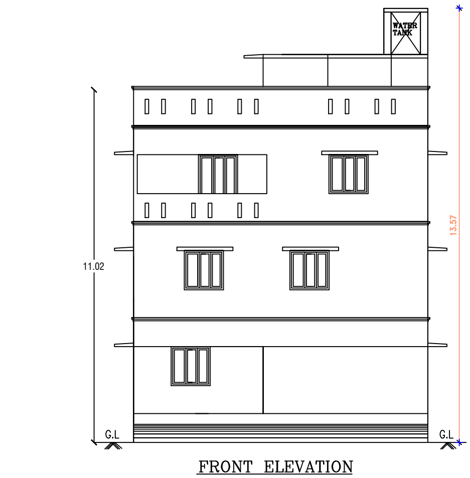
FRONT ELEVATION
