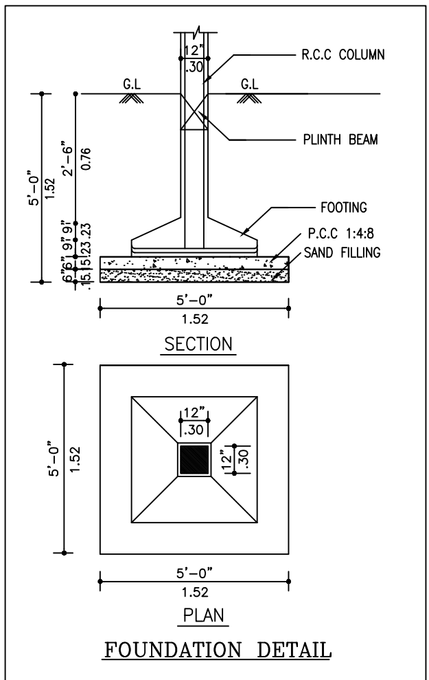
FOUNDATION DETAIL
