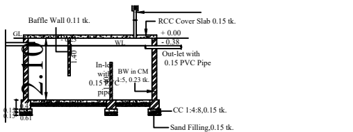
SECTION - SEPTIC TANK & SOAK PIT
