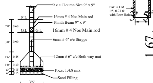
COLUMN DETIAL
