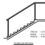
STAIRCASE DETAILS
