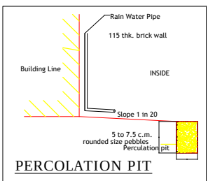
PERCOLATION PIT
