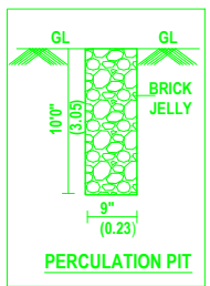
PERCOLATION PIT
