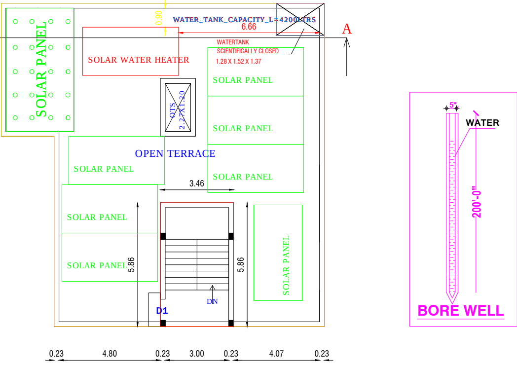
PRO. TERRACE FLOOR PLAN.
