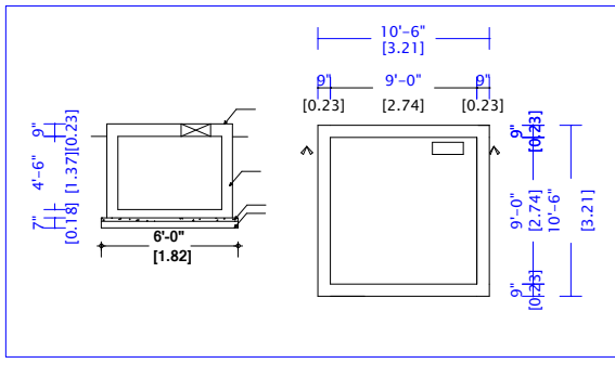
DETAILS OF FOUNDATION
