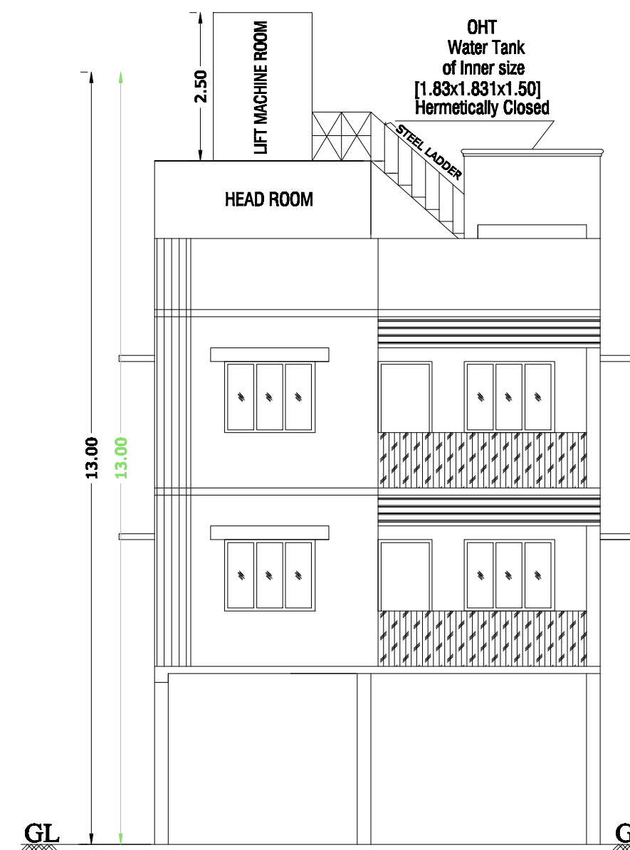
FRONT ELEVATION
