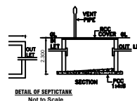
DETAIL OF SEPTIC TANK
