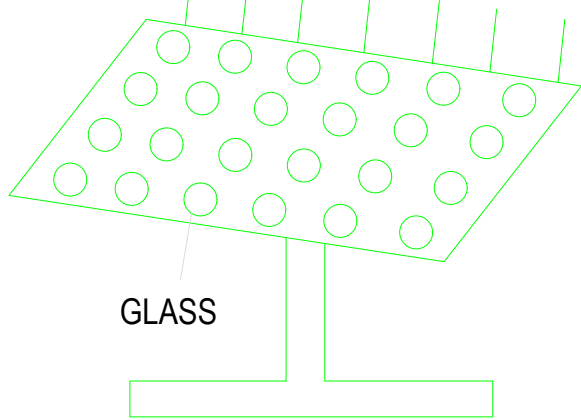
SOLAR SYSTEM
