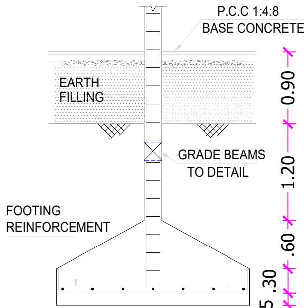
SECTION 'E-E'
