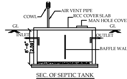
SEC. OF SEPTIC TANK
