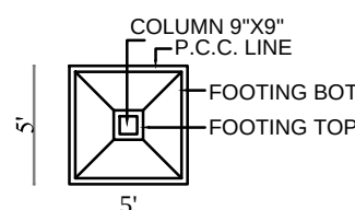
PLAN OF FOOTING
