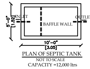
PLAN OF SEPTIC TANK
