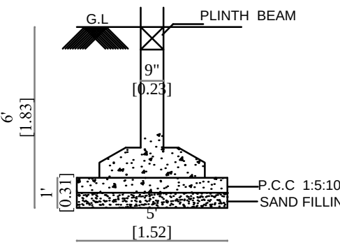
FOUNDATION DETAIL
