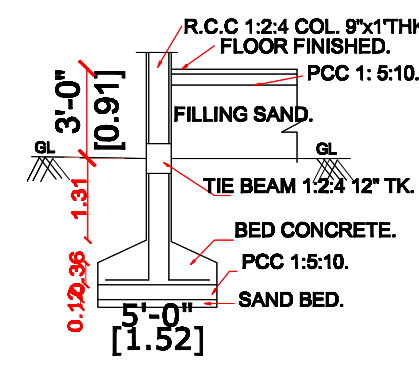
COLUMN FOUNDATION
