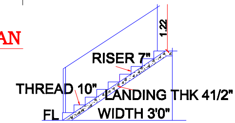
SEC. OF STAIR CASE DETAILS
