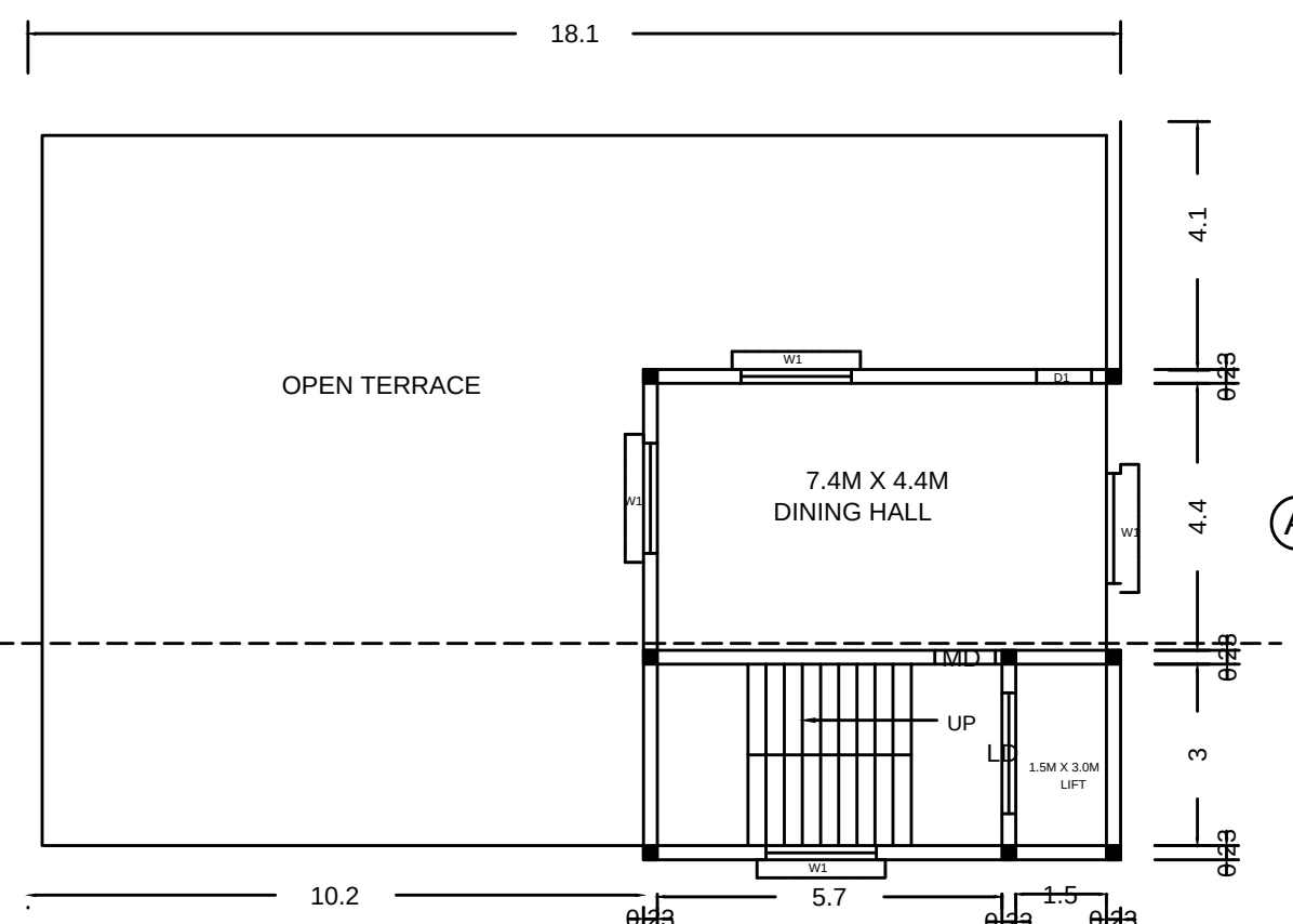
SECOND FLOOR PART PLAN (PROPOSED)
