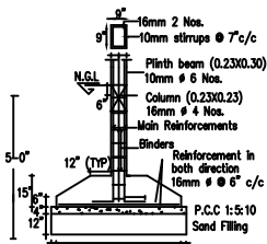
DETAILS OF FOUNDATION
