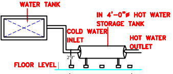
Solar Waterheater Detail
