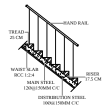
STAIR CASE PLAN (SCALE- 1:300)
